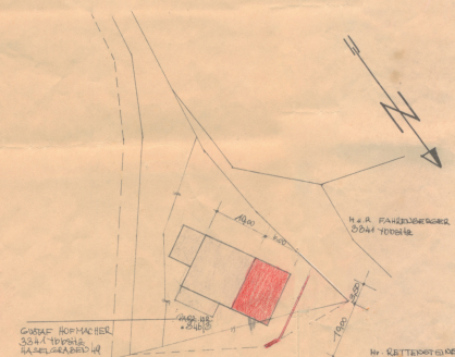
LAGEPLAN M = 1 : 500
